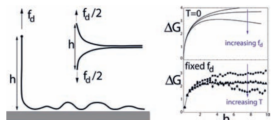
Fig. 1: Left: Force-induced desorption of an adsorbed filament and unzipping of two bound filaments. Right: Free energy landscapes for force-induced desorption as a function of the height h of the polymer end. The polymer desorbs either upon increasing the desorbing force f_d , or the temperature T . Both processes are governed by a free energy barrier.
