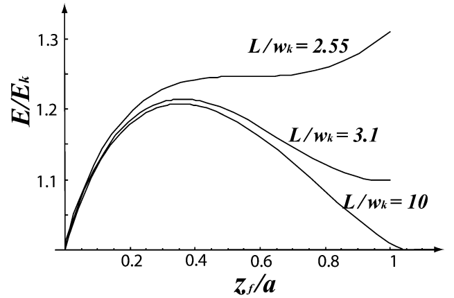
Fig. 3. Energy E_k(L/w_k, z_f/a) (in units of 2E_k ) of a “restricted” kink as a function of the end point z_f (in units of a ) and the kink-antikink distance L (in units of w_k ) for a semiflexible polymer of total length 2L . For distances L/w_k > 3.1 the kink is locally stable at z_f/a = 1 , for 2.55 < L/w_k < 3.1 the locally stable kink is obtained for z_f/a < 1 , and for L/w_k < 2.55 it becomes unstable.
