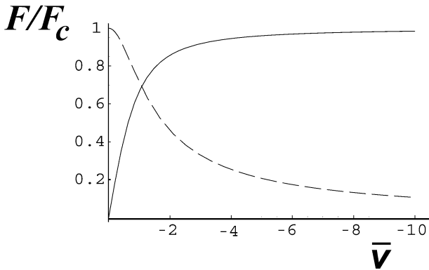
Fig. 5. Force density F (in units of F_c , solid line) and friction constant \eta_k (in units of 3F_c a / 2^{3/2} v_{sc} = 3a^2 \gamma / w_k , dashed line) as a function of velocity \bar{v} = 3^{3/4} v / 4v_{sc} for a moving kink.
